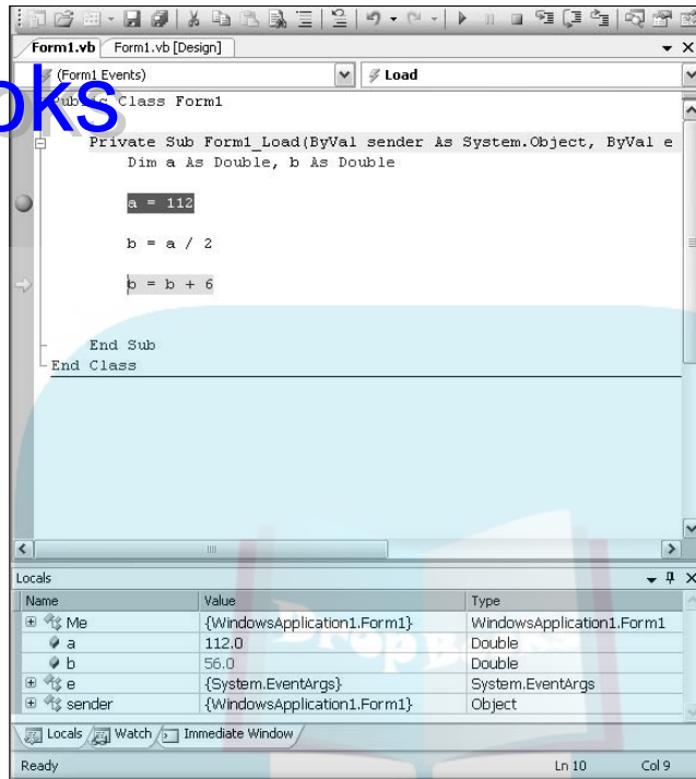
Figure 10-3: The Locals window displays the contents of all local variables in the currently executing procedure.
